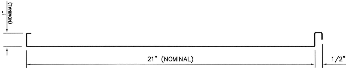
PANEL PROFILE
